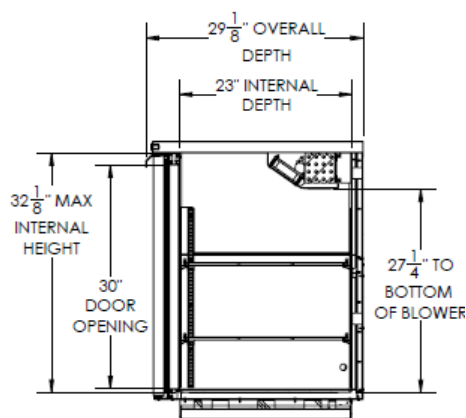
Elevation View
