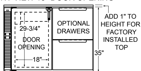
FRONT VIEW 18" DOOR OPENING
