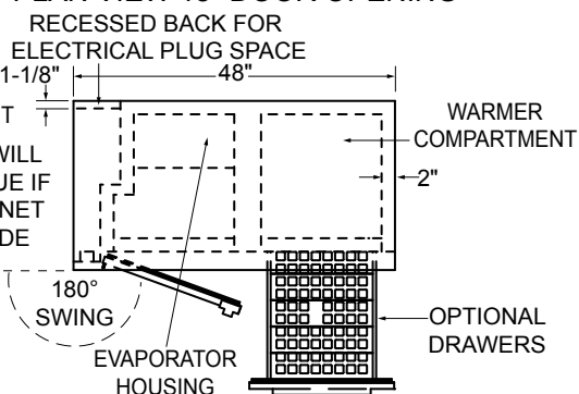
PLAN VIEW 18" DOOR OPENING
