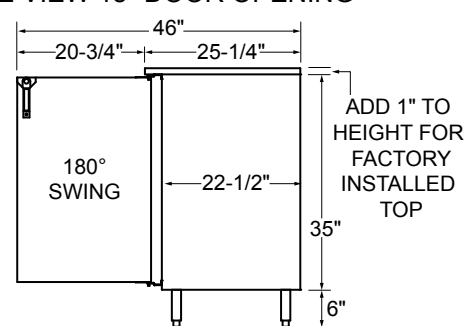
SIDE VIEW 18" DOOR OPENING
