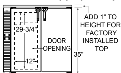
FRONT VIEW 12" DOOR OPENING
