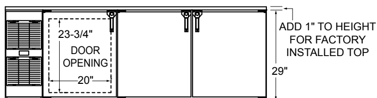
FRONT VIEW 20" DOOR OPENING
