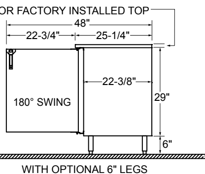
SIDE VIEW 20" DOOR OPENING
