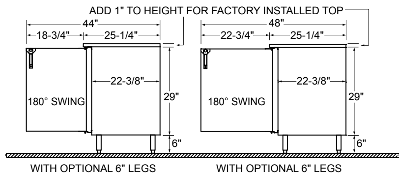
SIDE VIEW 16" DOOR OPENING
