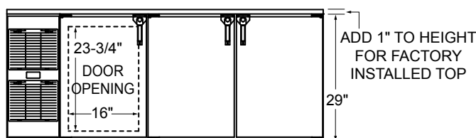
FRONT VIEW 16" DOOR OPENING
