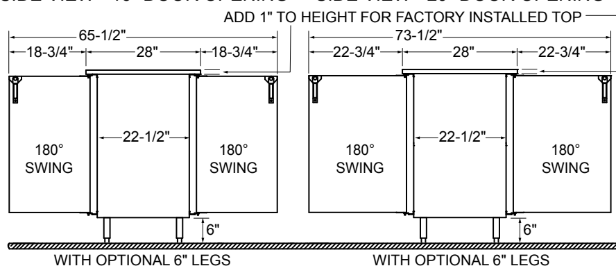
SIDE VIEW - 16" DOOR OPENING
