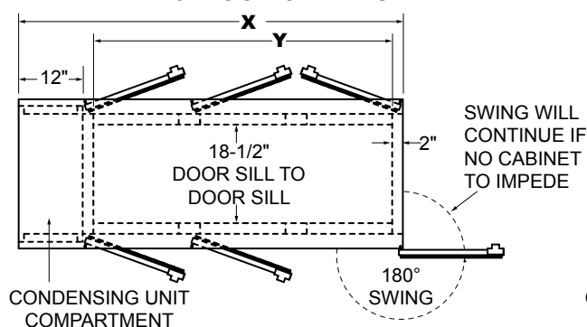
PLAN VIEW 16" DOOR OPENING
