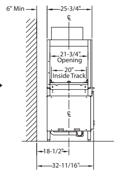
End View
